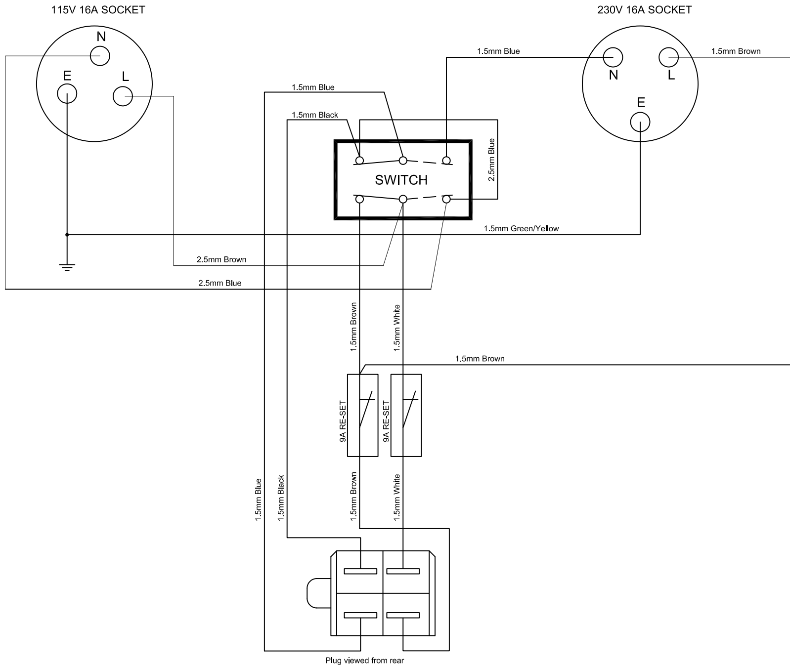
Plug viewed from rear
